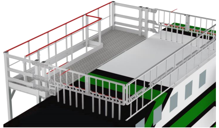
3D view of the deployable ring
